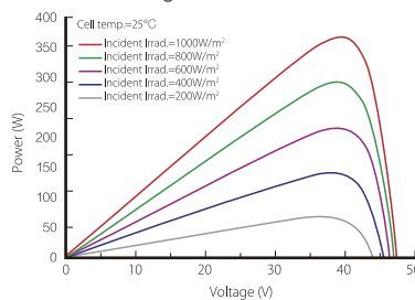
Power-Voltage Curve (LR6-72DG-335M)
