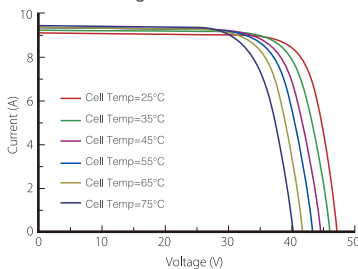
Current-Voltage Curve (LR6-72DG-335M)
