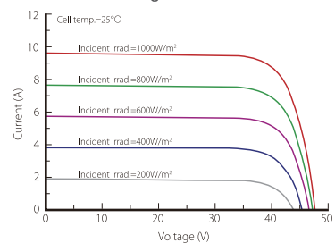
Current-Voltage Curve (LR6-72DG-335M)
