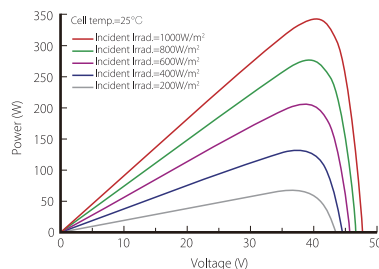
Power-Voltage Curve (LR6-72-335M)
