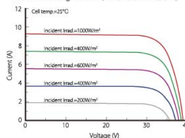
Current-Voltage Curve (LR6-60BK-280M)
