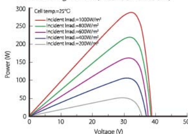
Power-Voltage Curve (LR6-60BK-280M)
