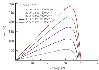
Power-Voltage Curve (LR6-60-285M)
